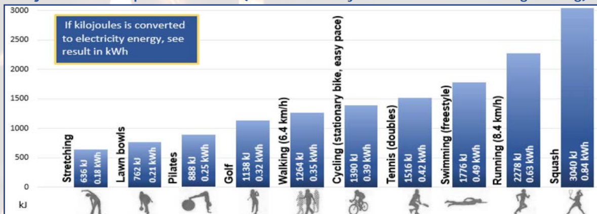
Kilojoules burned per 60 minutes (based on a 40 year-old woman who weighs 70kg)
